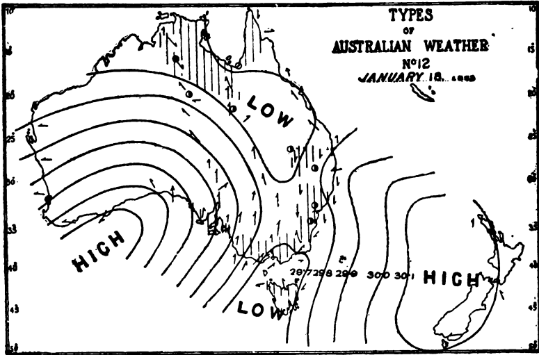
TYPE VI.—CYCLONIC THUNDERSTORMS.
